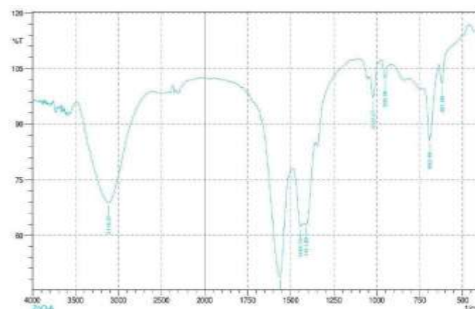
Fig. 3: FTIR Spectrum of ZnO NP's synthesized from Calotropis procera
